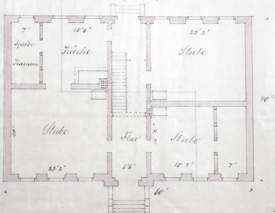
Rycina 79. Rzut parteru willi Johanna Quistorpa, 1865, APS, AMSPB, 15876
